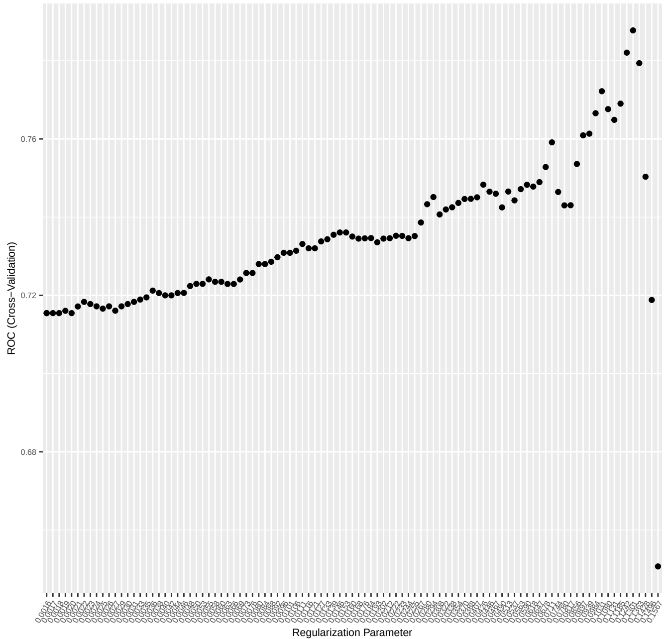
lasso Model using caret package:Microbiome Species Abundance Data;1981 Microbiome species,187 Pati
